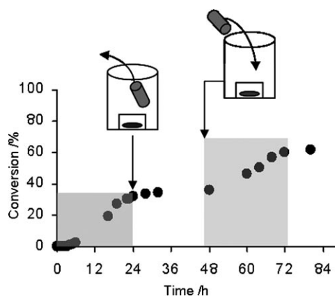
Figure 3. Stepped reaction profile for acetophenone conversion, showing the removal and replacement of the membrane cup at 24 h intervals. Reaction conditions: acetophenone (0.23 mL, 2 mmol), pentadecane (internal standard, 1 mmol), and i PrOK (0.1 mL, 10 mmol) stirred under \text{N}_2 in i PrOH (20 mL) at 25 °C under nitrogen.
